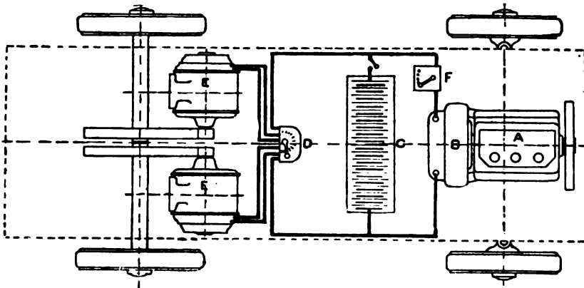
FIG. 428.—The Fischer Electric Omnibus, driven by dynamo direct. A is the gasoline engine, driving the dynamo, B; C, the storage battery; D, the switch; E, E, motors; F, rheostat.
